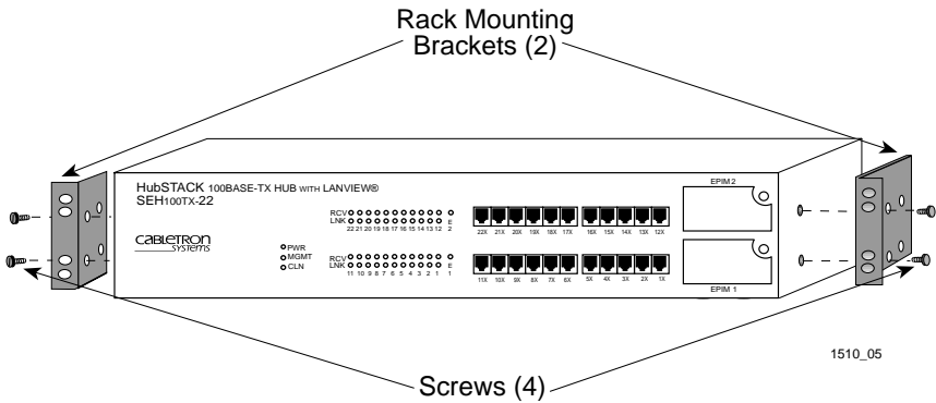
Figure 4-3 Installing the Rack Mounting Brackets
